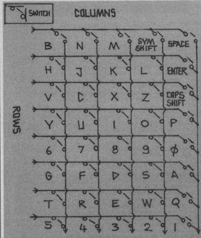
Figure 1 The Spectrum keyboard unmasked
